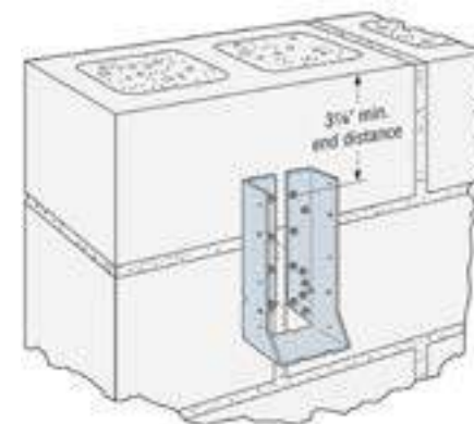
SIMPSON STRONGTIE HUC JOIST HANGERS
