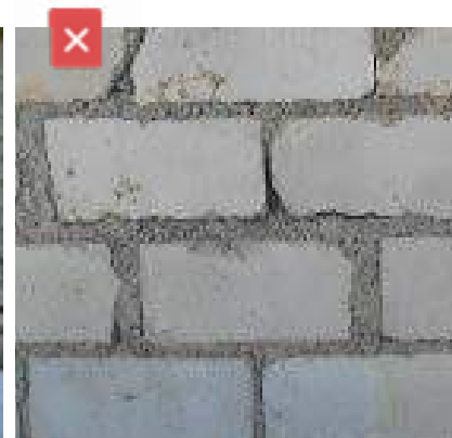
Mortar joints too thick
